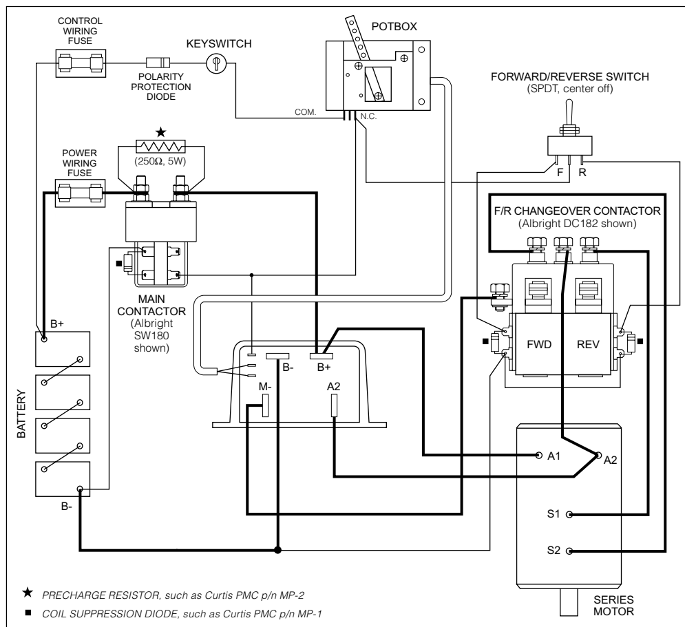
Fig. 5 Typical installation, Curtis PMC 1204/1205 controller.
