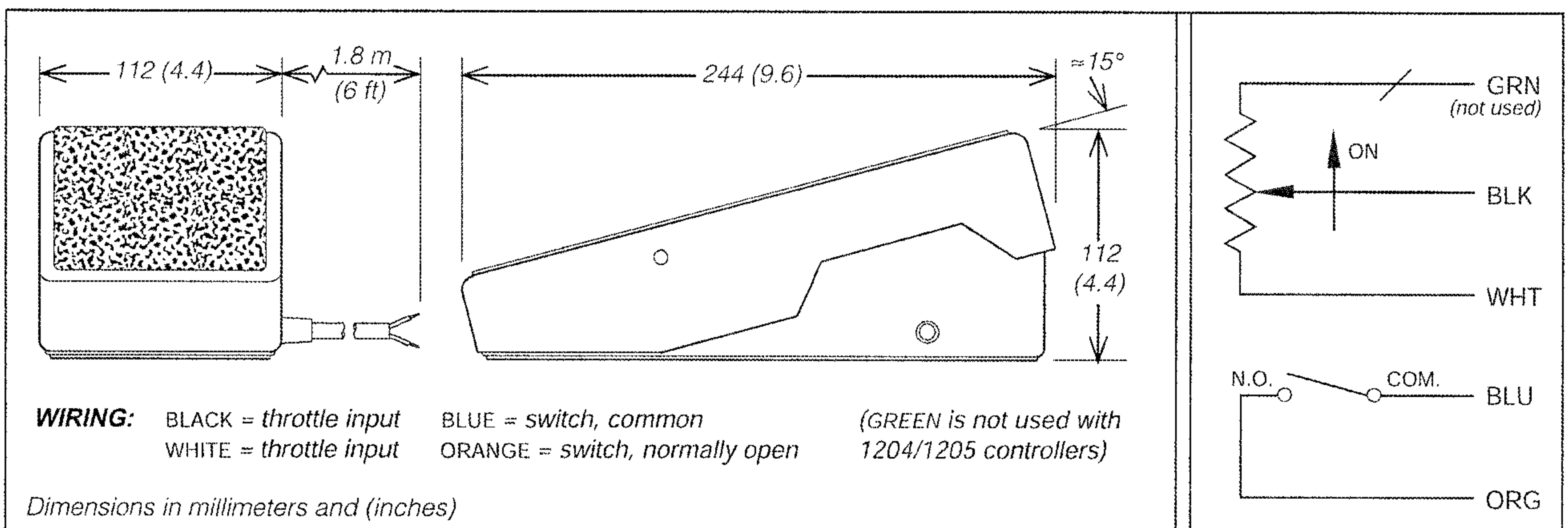
Fig. 4 Curtis PMC footpedal FP-2.
